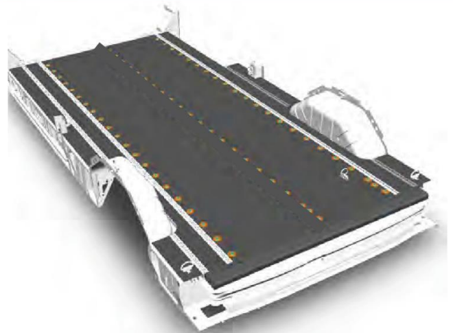
4 rows of L-TRACKS with 3-rows of Roller Panels
